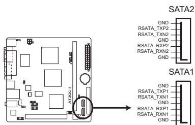
AT3GC-I SATA connectors
