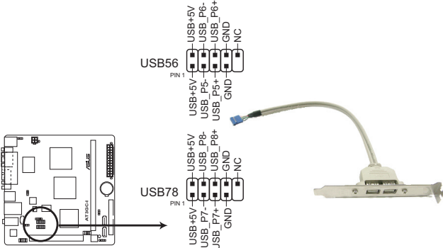
AT3GC-I USB2.0 connectors
