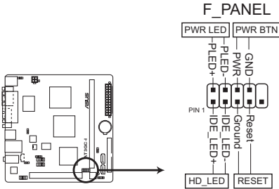
AT3GC-I System panel connector
