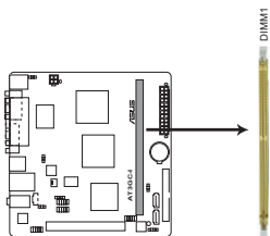
AT3GC-I 240-pin DDR2 DIMM socket
