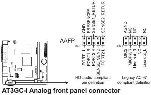
AT3GC-I Analog front panel connector
