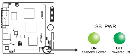
AT3GC-I Onboard LED
