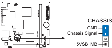
AT3GC-I 240-pin Chassis intrusion connector
