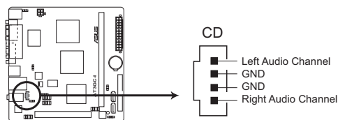
AT3GC-I Internal audio connector
