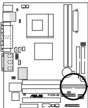
TUSI-M Floppy Disk Drive Connector
