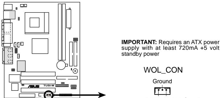
TUSI-M Wake-On-LAN Connector
