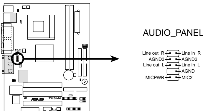
TUSI-M Audio Panel Connectors
