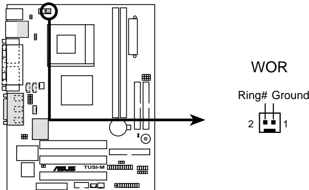
TUSI-M Wake On Ring Connector
