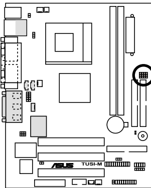
TUSI-M CPU External Frequency Selection
