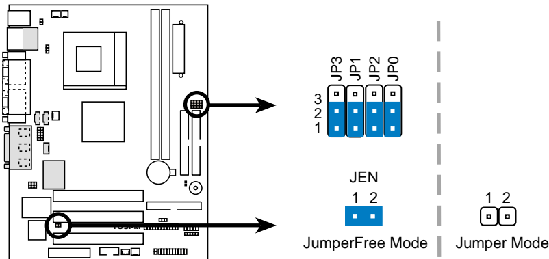
TUSI-M JumperFree™ Mode Setting
