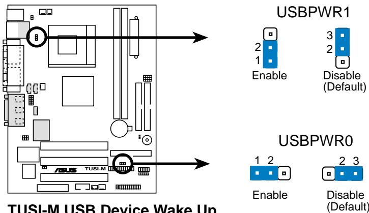
TUSI-M USB Device Wake Up
