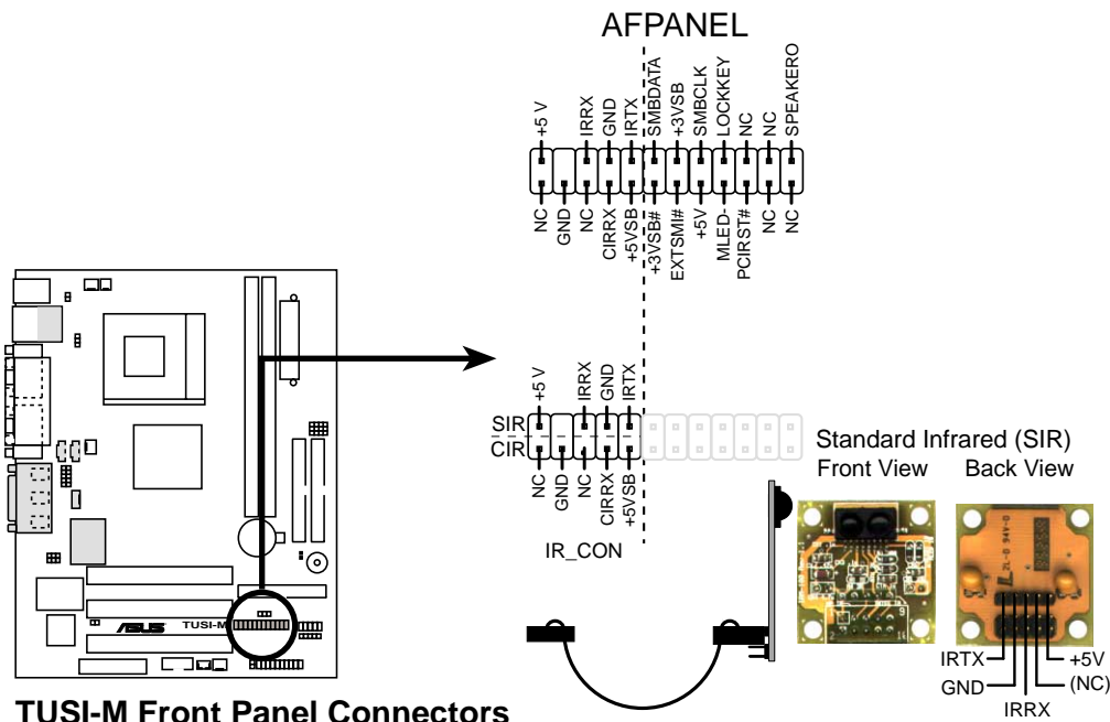
TUSI-M Front Panel Connectors
