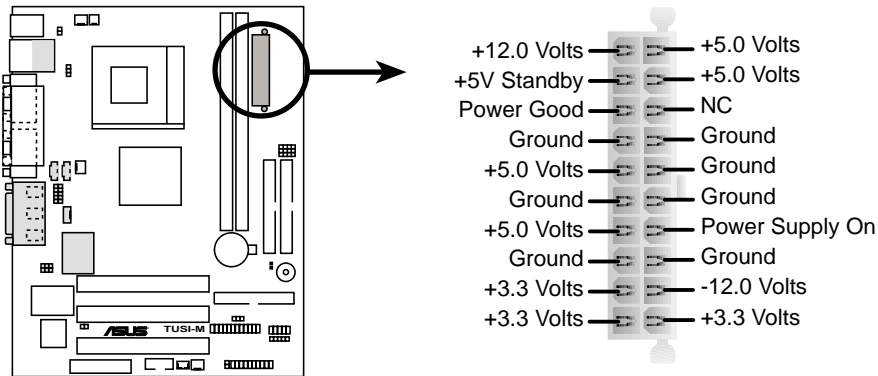
TUSI-M ATX Power Connector
