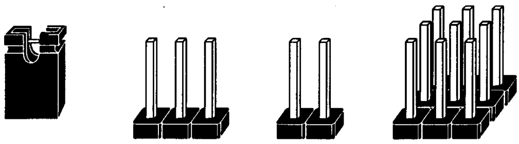
Jumper cap 3-pin jumper 2-pin jumper Jumper block
